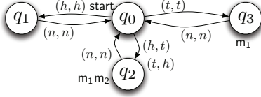
Figure 1: A simple CGS \mathfrak{M}_0 .
