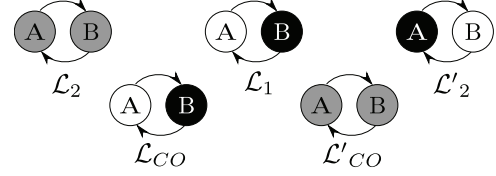
Figure 3: The credulous operator is not strategy-proof.
