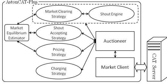
Figure 1: AstonCAT-Plus architecture.
