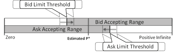
Figure 2: General structure of AstonCAT-Plus's accepting strategy. Shaded areas are accepting ranges. The arrows pointing to the equilibrium price line indicate directions by which accepting thresholds shift during a day.
