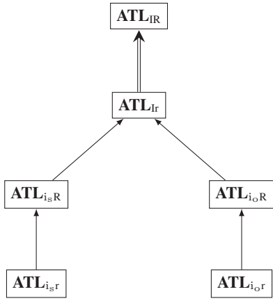
Figure 5: Summary: comparison of validity sets induced by various semantics of ATL. The arrows denote strict subsumption, i.e. L_1 \rightarrow L_2 means that Val(L_1) \subsetneq Val(L_2) . Unconnected pairs of nodes correspond to logics with incomparable validity sets. The double line indicates that the IR and Ir semantics induce the same validities in “vanilla” ATL, but different in the broader languages ATL^+ and ATL^* .
