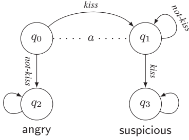
Figure 4: Model M_4 with \text{Agt} = \{a\} : dangers of marital life
