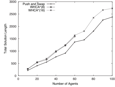
Figure 8: The average total solution length computed by the WHCA and PUSH_AND_SWAP approaches in the random placement problems. Values are averages of 20 runs.
