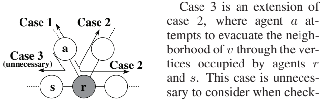
Figure 3: The three cases considered when evacuating a from the neighborhood of v (shaded).
