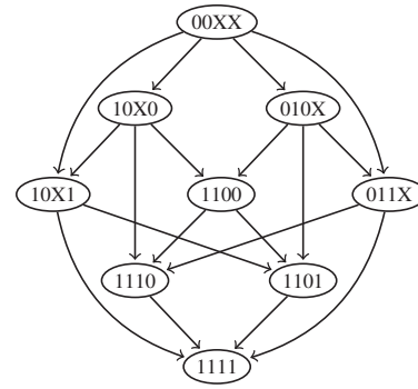
Figure 2: Families of seeding restrictions. Each label is a four tuple where 1 means fixed, 0 means unfixed and X is a don't care value. Don't care values are used to denote when the models are solution equivalent. The four tuple values represent are, from left to right, pooling, team arrangement, team ranking and pool arrangement.
