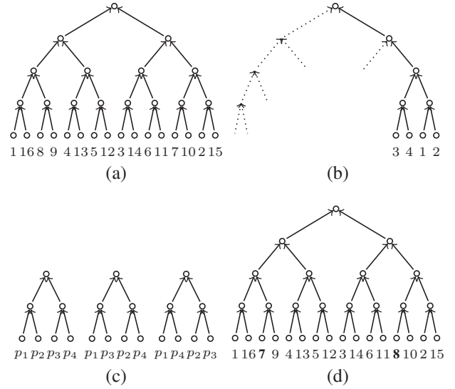
Figure 1: (a) The arrangement of teams by rank used by the NCAA Division I Basketball Championship. The numbers below the leaf nodes represent the rank of the team at that leaf. (b) A seeding can be manipulated so that all of the top teams play each other in the first two rounds. (c) The possible ways that the winners of the four pools of the NCAA could be arranged. (d) Changing the rank of a team from eight to seven can completely change their opponents.
