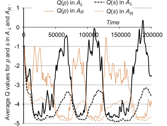
Figure 6: Average Q values in state S for actions p and s in A_L and A_R with self-centered agents.
