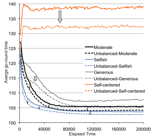
Figure 8: Average go-round times over times (unbalanced populations).
