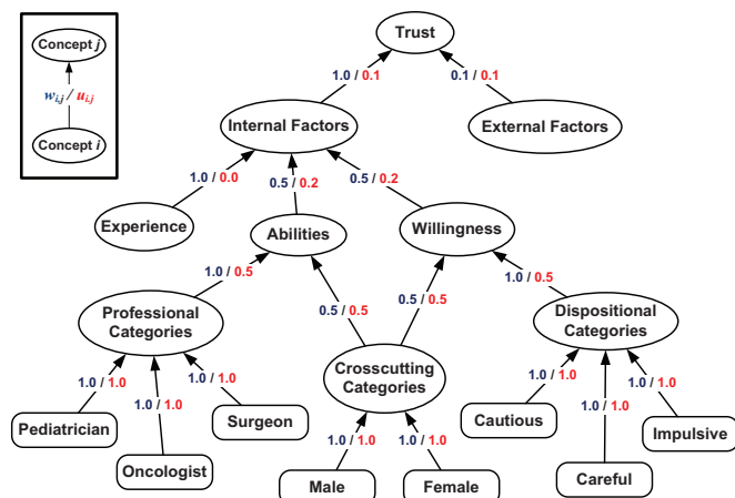
Figure 1: UnFCM implementing socio-cognitive trust
