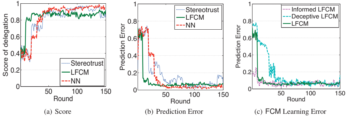
Figure 2: Score chart (a) and error charts (b,c) for different trustors approaches.
