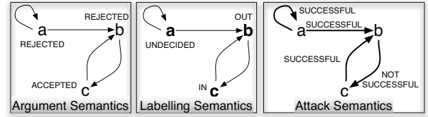
Figure 1: Successful attacks by in and undecided arguments.
