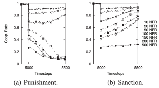
Figure 2: New Free Riders introduced at TS = 5000.
