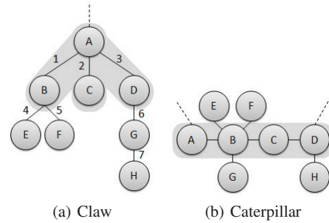
Figure 1: Self-Reinforcing Structures.
