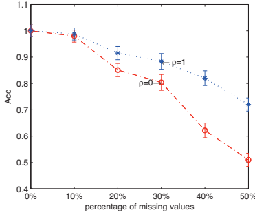
Figure 2: The recognizing accuracy with respect to different percentages of missing values ( M is set to be 80)
