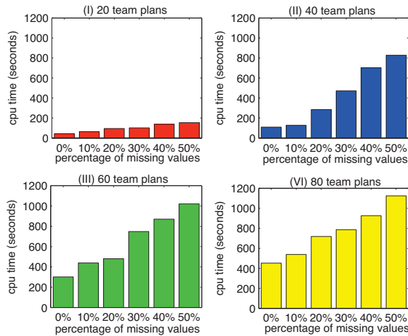
Figure 4: CPU time with respect to different percentages of missing values.
