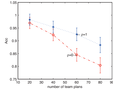
Figure 3: The recognizing accuracy with respect to different numbers of team plans ( \xi is set to be 30%)
