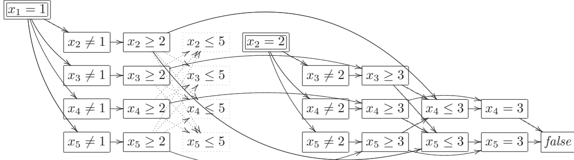
Figure 1: Implication graph of propagation. Decision literals are double boxed.
