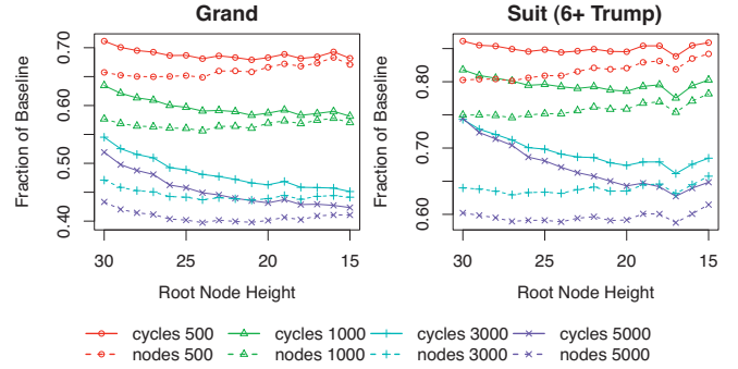
Figure 2: Reduction in nodes and search times using precomputed transposition tables of various sizes.
