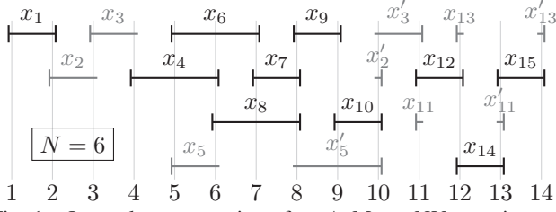
Fig. 1: Interval representation of an ATMOST-NVALUE instance \mathcal{I} = (X, D, \text{dom}, N) , with X = \{x_1, \dots, x_{15}\} , N = 6 , D = \{1, \dots, 14\} , and \text{dom}(x_1) = \{1, 2\} , \text{dom}(x_2) = \{2, 3, 10\} , etc.
