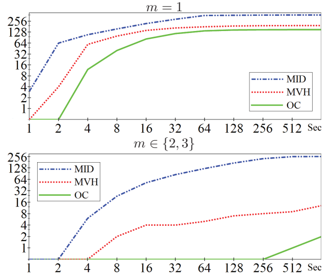
Figure 1: Number of solved problems vs time.
