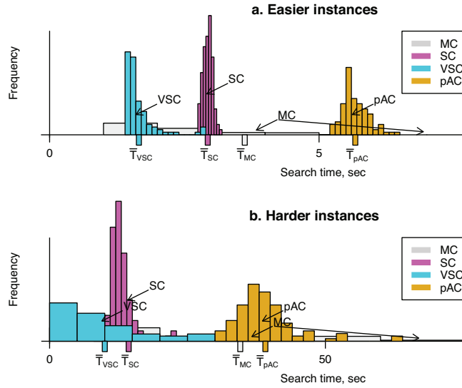
Figure 2: Search time comparison on sets of random instances (using Model RB)
