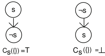
Figure 1: AFs simulating C_s(\emptyset) \in \langle \top, \perp \rangle
