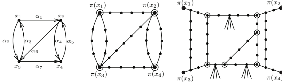
Figure 1: From left to right: an example query Q_1 (an arc x \rightarrow y labeled with \alpha stands for the atom \alpha(x, y) ); the (classic) structure of a counter-example \mathcal{I} for Q_1 \subseteq Q_2 , for some (in this context irrelevant) query Q_2 , in the absence of constraints (4 split points corresponding to V(Q_1) ); and a possible structure of \mathcal{I} in the presence of DL constraints (6 split points, tree-shaped structures attached).
