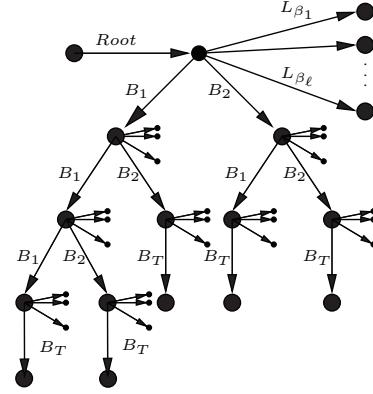
Figure 3: Example structure without structural errors ‘generated’ by the query Q_1 in Figure 2, for the case where m = 2 .
