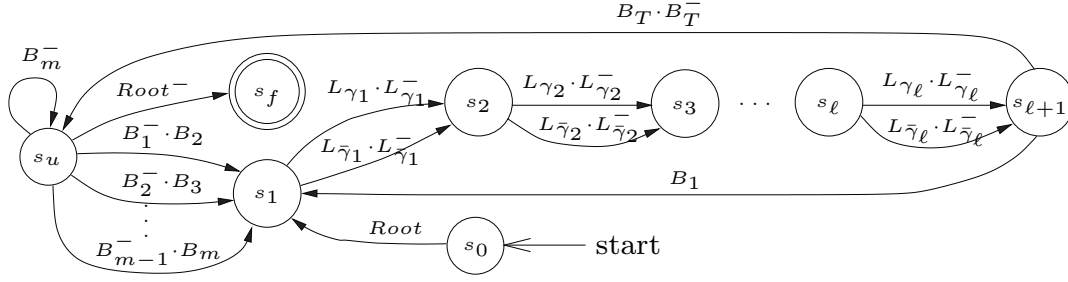
Figure 2: The automaton for the query Q_1(x, y) \leftarrow \alpha_1(x, y) .
