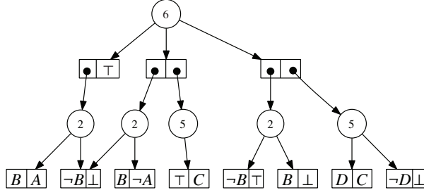
Figure 2: An SDD for f = (A \wedge B) \vee (B \wedge C) \vee (C \wedge D) , which is normalized for v = 6 in Figure 1(a).
