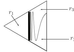
Figure 1: Three regions in \text{RC}(\mathbb{R}^2) satisfying (2).
