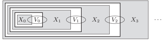
Figure 3: The sequence \{X_i, V_i\}_{i \geq 0} generated by \varphi_\infty . ( S_{i+1} and R_{i+1} are the ‘holes’ of X_{i+1} containing X_i and X_{i+2} .)
