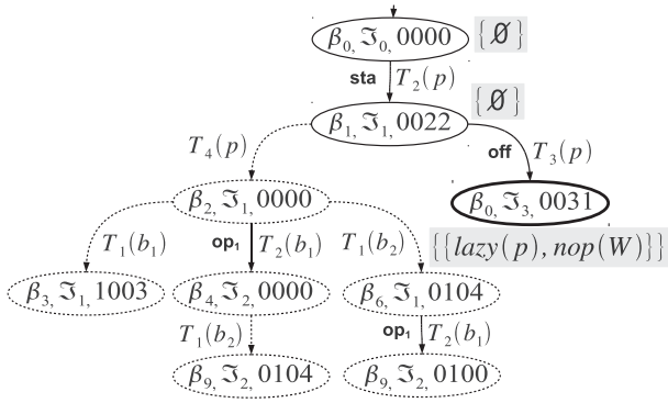
Figure 6: Behavior Bhv(\varphi(W)) .
