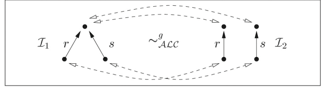
Figure 5: Globally bisimilar interpretations
