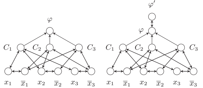
Figure 4: Illustrations for the reductions in proof of Theorem 5. (F, \varphi) and (F', \varphi') are instances of \text{CA}_\sigma and \text{SA}_\sigma , respectively, obtained from the 3-CNF formula \varphi = C_1 \wedge C_2 \wedge C_3 with C_1 = x_1 \vee x_2 \vee x_3 , C_2 = \neg x_1 \vee x_2 \vee \neg x_3 and C_3 = \neg x_1 \vee \neg x_2 \vee \neg x_3 . The set \{\varphi\} is a SYM-backdoor for F and F' .
