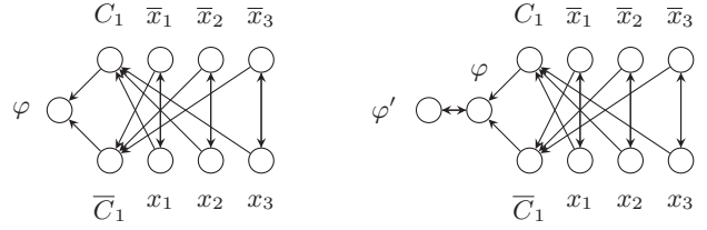
Figure 3: Illustrations for the reductions in the proof of Theorem 4, showing instances (F, \varphi) and (F', \varphi') for the problems \text{CA}_\sigma and \text{SA}_\sigma , respectively, obtained from the monotone 3-CNF formula \varphi = C_1 \wedge \bar{C}_1 with C_1 = x_1 \vee x_2 \vee x_3 and \bar{C}_1 = \neg x_1 \vee \neg x_2 \vee \neg x_3 . The set \{\varphi\} is a BIP-backdoor for F and F' .
