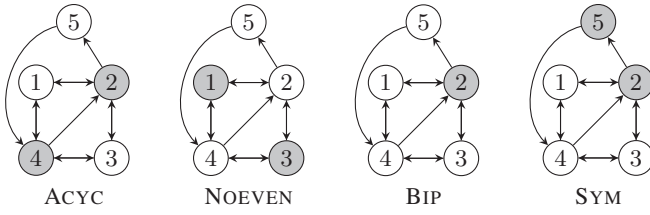
Figure 2: Backdoors for the AF F from Example 1, with respect to the indicated classes.
