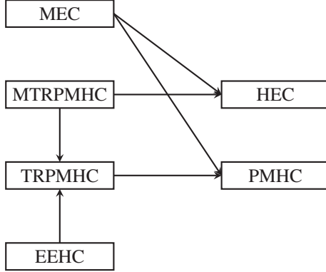
Figure 1: Relationships between Horn contractions.
