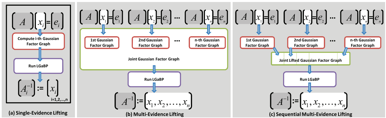
Figure 2: Inverting a matrix \mathbf{A} using multi-evidence lifting. (a) Single-evidence lifting runs LGaBP solving \mathbf{A}\mathbf{x}_i = \mathbf{e}_i for each i = 1, 2, \dots, n separately; \mathbf{e}_i denotes the i th basis vector; thus LGaBP computes each column vector of \mathbf{A}^{-1} separately. (b) Multi-evidence lifting runs LGaBP on the joint graphical model of \mathbf{A}\mathbf{x}_i = \mathbf{e}_i for i = 1, 2, \dots, n ; thus LGaBP computes \mathbf{A}^{-1} for all \mathbf{e}_i at once. (c) Sequential multi-evidence lifting directly builds the lifted joint graphical model in a sequential fashion, avoiding cubic space complexity
