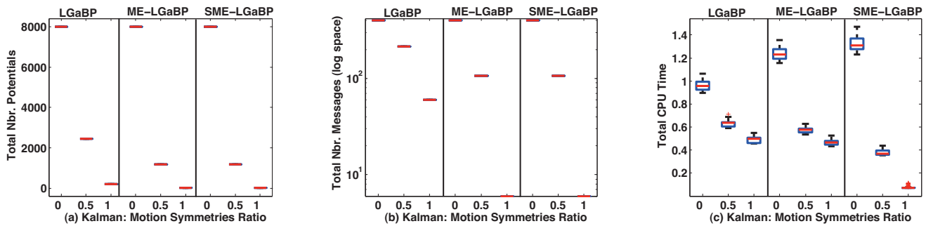
Figure 4: Experimental results for Kalman filtering with varying degree of motion symmetries. (best viewed in color)
