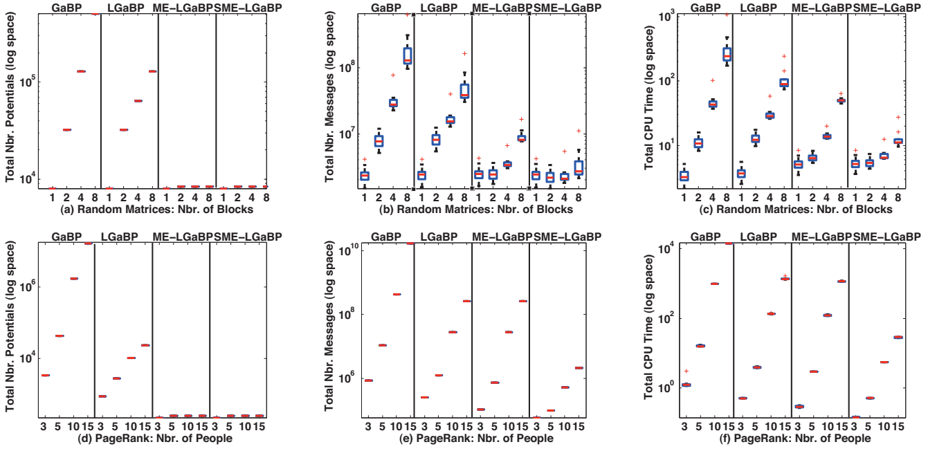
Figure 3: Experimental results on random matrices and PageRank computations. (best viewed in color)
