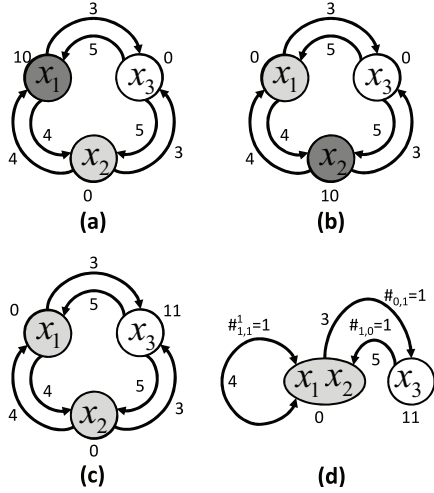
Figure 1: Lifted graphical models produced when inverting \mathbf{A} in Eq. (1) using LGaBP. An edge from i to j encodes potential \psi_{ij} . The \phi potentials are associated with the nodes. (a) Colored network when computing \mathbf{A}\mathbf{x}_1 = \mathbf{e}_1 . All nodes get different colors; no compression and lifted inference is essentially ground. (b) Colored network for \mathbf{A}\mathbf{x}_2 = \mathbf{e}_2 . Again no compression. Note, however, the symmetries between (a) and (b). (c) Colored network for \mathbf{A}\mathbf{x}_3 = \mathbf{e}_3 . Nodes x_1 and x_2 get the same color and are grouped together (d).
