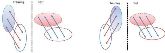
Figure 3: Case one: There exists significant covariate shift in \Pr(x) but not in Q(\delta_x) . Case two: There exists significant covariate shift in \Pr(x) as well as in Q(\delta_x) .
