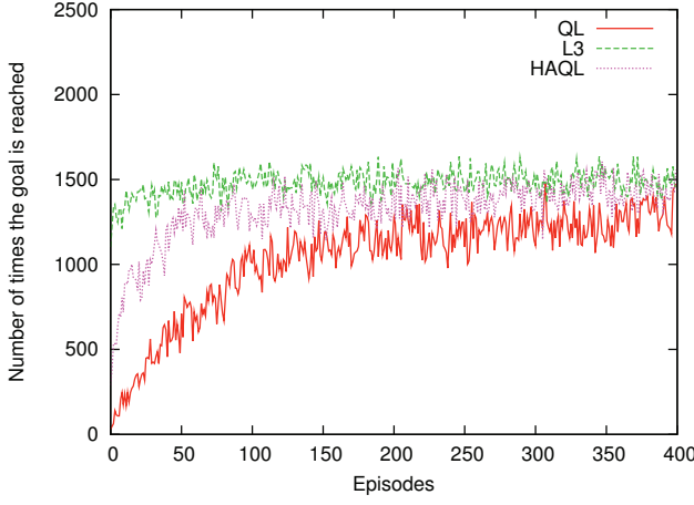
Figure 3: The learning curves for the Q -learning, HAQL and L3 algorithms
