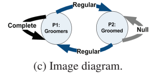
Figure 1: Adjacency matrix and image matrix and diagram for the Baboon grooming network.
