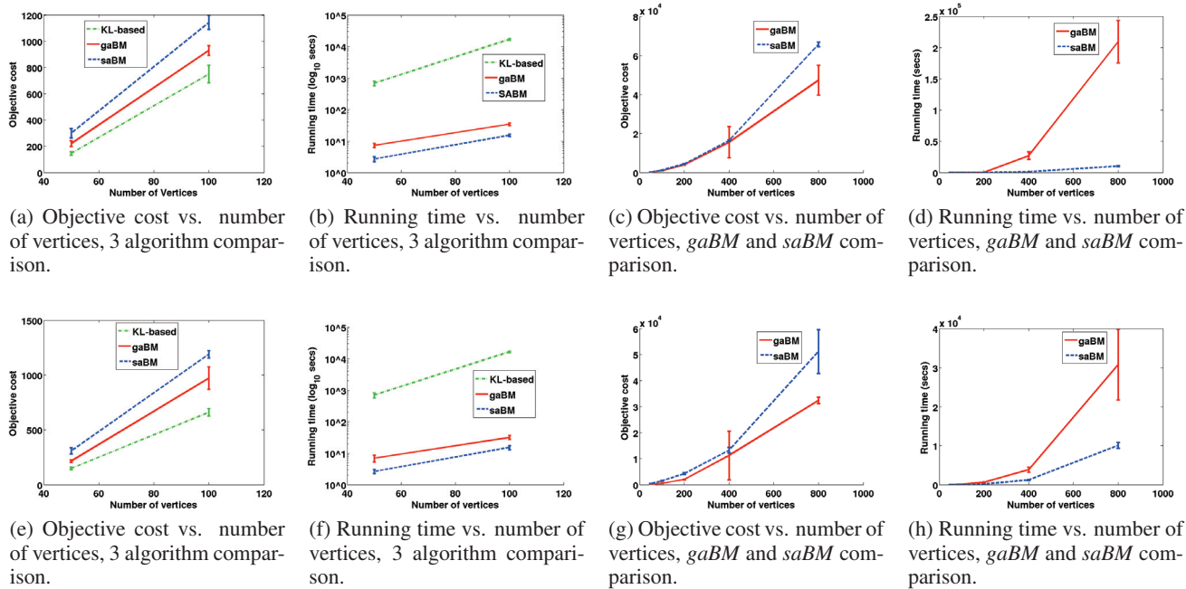
Figure 4: Objective cost and running time results for the generated community datasets. Top row of figures: No Blockmodel supplied. Bottom row: Blockmodel supplied.
