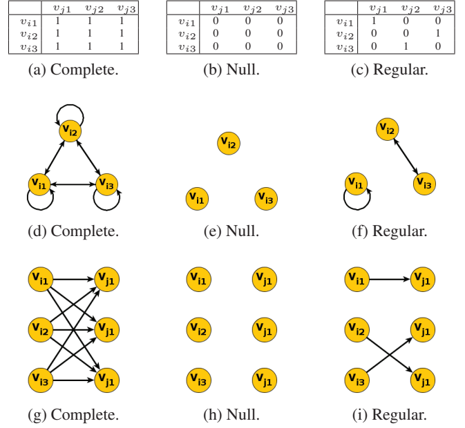
Figure 2: Three block types and their ideal adjacency and block patterns. The example for the regular type is just one possibility. First row is the adjacency matrix, second and third row are the graph representation for diagonal and non-diagonal blocks respectively.
