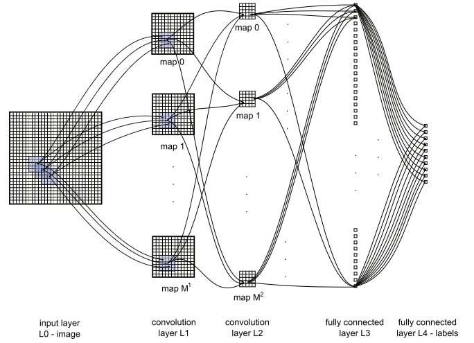
Figure 1: Architecture of a convolutional neural network with fully connected layers, kernel sizes of 5 x 5 and skipping factors of 1.
