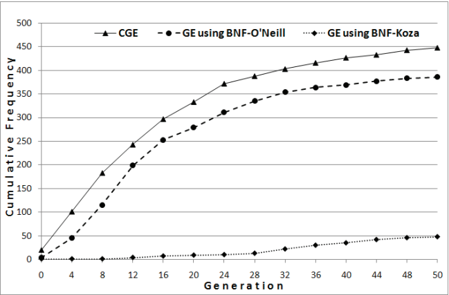
Figure 9: CGE vs. GE on the Santa Fe Trail problem.
