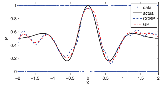
Figure 5: Estimated probability after 1000 observations.
