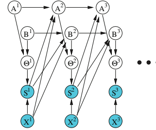
Figure 4: DBN model to learn multivariate beta distributions.
