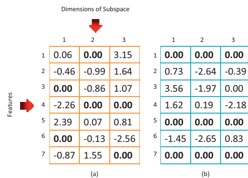
Figure 1: An illustrative toy example of the projection matrices learned by (a) Sparse subspace learning; and (b) feature selection and subspace learning
