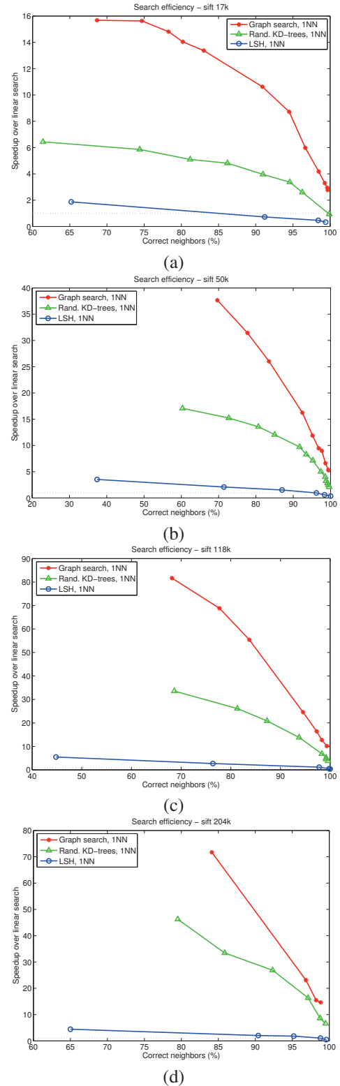
Figure 3: The results for a NN search problem ( K = 1 ). Speedup vs. accuracy for different algorithms (GNNS, randomized KD-tree, and LSH) on datasets of (a) 17k (b) 50k (c) 118k (d) 204k points. The GNNS algorithm outperforms the two other methods. The gray dashed line indicates the speedup of 1.
