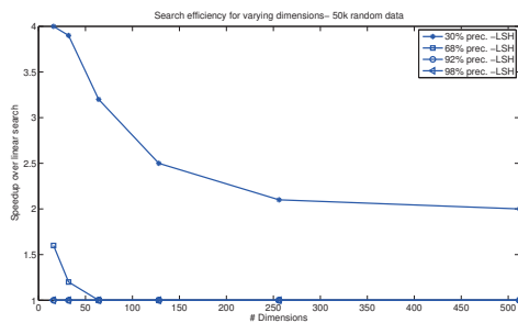
Figure 7: The results for a NN search problem ( K = 1 ). Speedup vs. dimension for different precisions for LSH algorithm. Datasets have 50k points.
