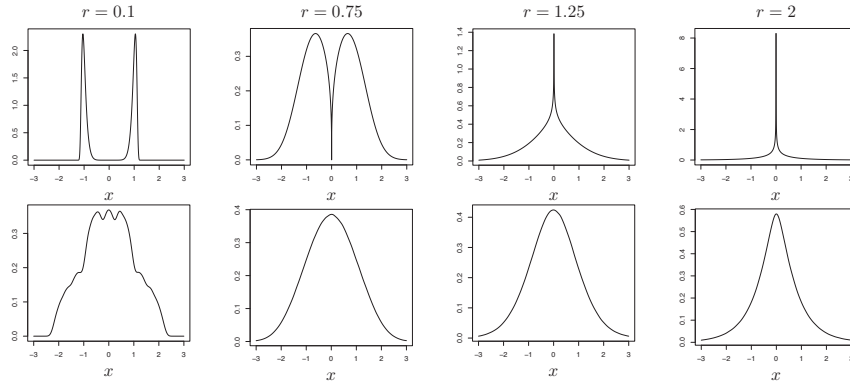
Figure 2: Density for the noise (top row) and the reversed residuals (bottom row) in an AR(1) model with \phi = (\sqrt{5} - 1)/2 .
