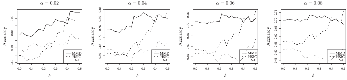
Figure 4: Results obtained by each method in the experiments with EEG data.
