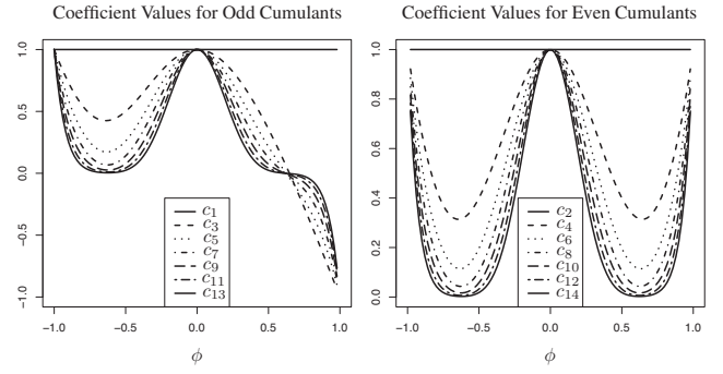
Figure 1: Coefficients c_n(\phi) (odd in the left plot, even in the right plot) in a causal AR(1) process.
