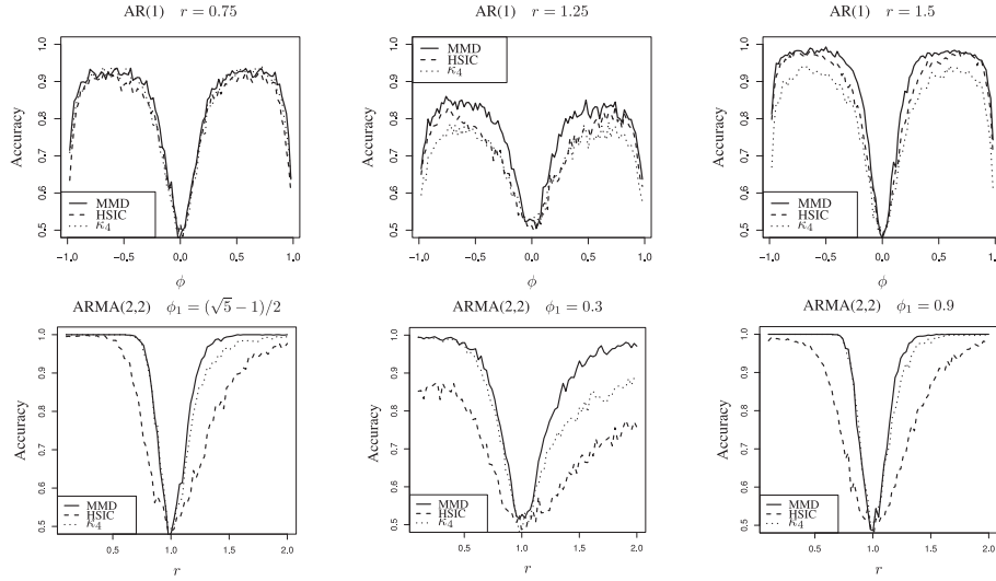
Figure 3: Results obtained by each method in the experiments with AR(1) and ARMA(2,2) time series.
