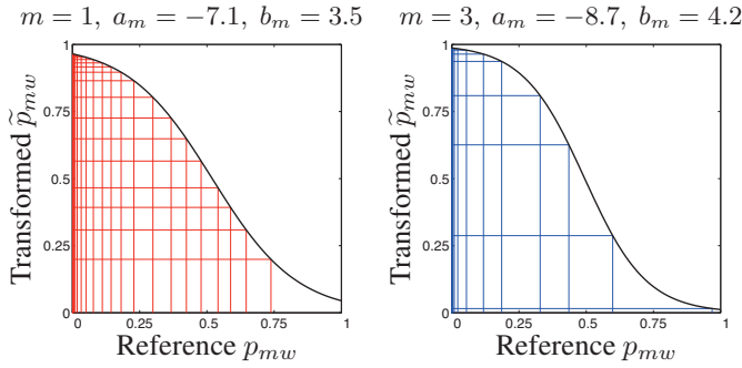
Figure 3: MNIST: estimated sigmoids for two of the components. The vertical and horizontal lines indicate pairs (p_{mw}, \tilde{p}_{mw}) (not all W pairs are shown, to avoid clutter). Note how both essentially invert the input.
