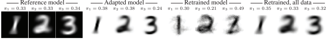
Figure 2: MNIST: MMB parameters for the reference model, adaptation (with N = 100 adaptation points), retraining (with N = 100 ) and retraining (with N = 18\,000 ).
