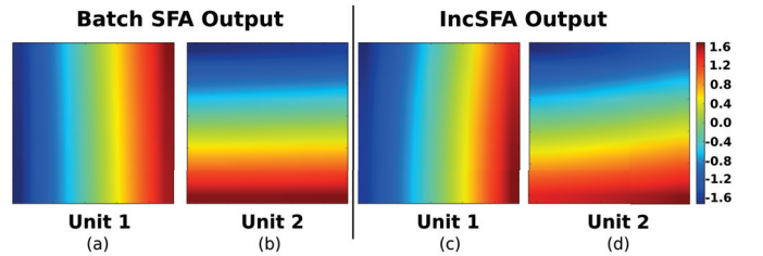
Figure 3: (a) Batch SFA output of the first slow feature and (b) the second slow feature (c) IncSFA output of the first slow feature and (d) the second slow feature after 50,000 samples with a learning rate \eta = 0.003 . Figures best viewed in color.
