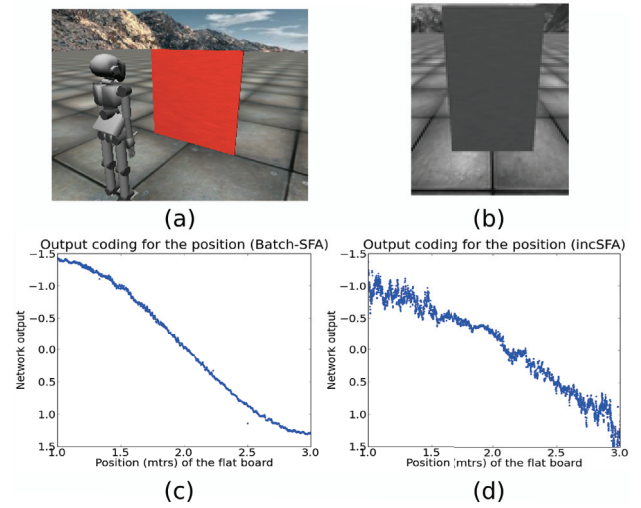
Figure 4: (a) Experimental Setup: iCub Simulator (b) Sample image from the input dataset (c) Batch-SFA output (d) IncSFA output ( \eta = 0.005 )
