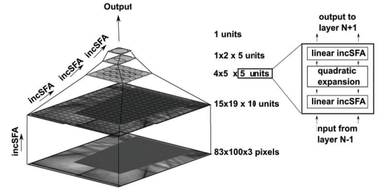
Figure 5: Hierarchical-Network Architecture
