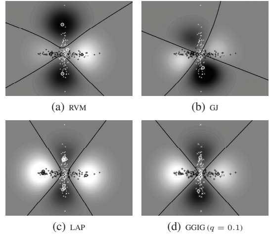
Figure 2: Experimental results in the cross data.
