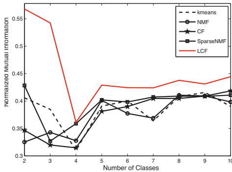
Figure 2: Mutual Information on the Yale database
