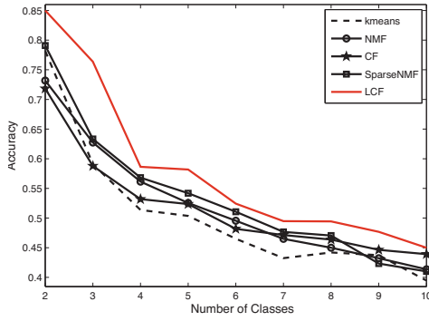
Figure 1: Accuracy on the Yale database
