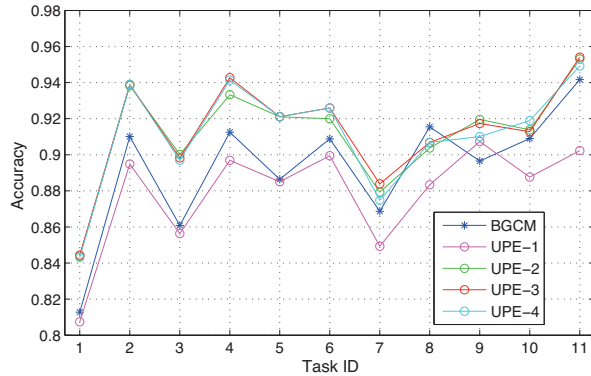
Figure 3: The accuracy of BGCM and UPE- D .
