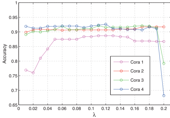
Figure 4: The accuracy on Cora data set with different \lambda value.
