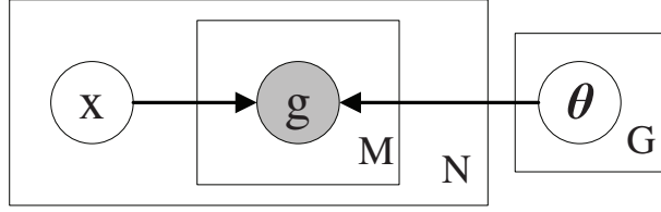
Figure 2: The Graphical Model of UPE
