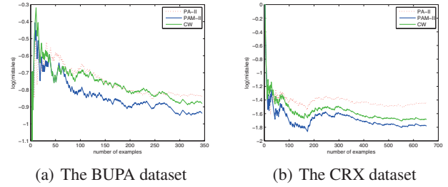
Figure 1: Cumulative error for BUPA and CRX.
