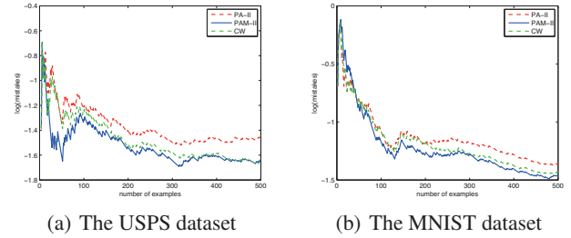
Figure 2: Cumulative error rate for USPS and MNIST.
