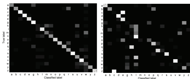
Figure 4: Confusion matrix showing performance of CSTM (left) and CSTM-DTW (right) on the character data.
