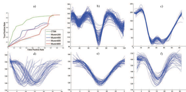
Figure 5: a) ROC curve for bradycardia, b-c) novel physiological markers recovered by CSTM, d) an example bradycardia cluster recovered by CSTM, e) aligned version of cluster in d, and f) an example bradycardia cluster from Mueen
