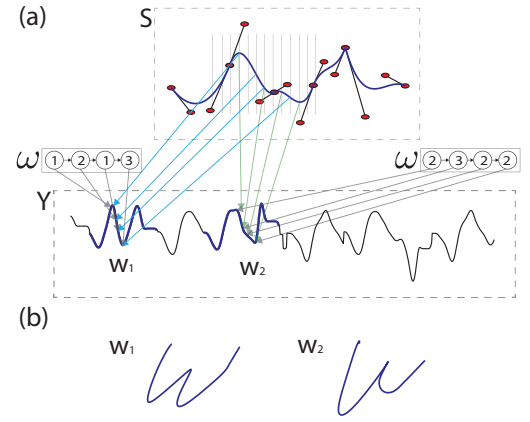
Figure 1: a) The template S shows the canonical shape for the pen-tip velocity along the x-dimension and a piecewise Bézier fit to the signal. The generation of two different transformed versions of the template are shown; for simplicity, we assume only a temporal warp is used and \omega tracks the warp at each time, b) The resulting character ‘w’ generated by integrating velocities along both the x and y dimension.
