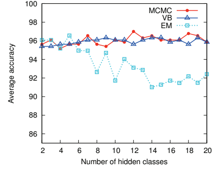
Figure 8: Average accuracy
