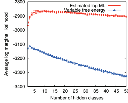
Figure 7: Average log marginal likelihood
