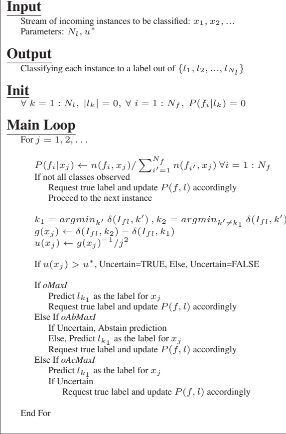
Figure 2: Pseudo-code for all three online classification algorithms proposed in this work. For the classical online setup, oMaxI is TRUE. For the algorithm with an abstain option, oAbMaxI is TRUE. For the active-learning algorithm, oAcMaxI is TRUE. The first “If” statement in the main “For” loop guarantees that the true label is always requested until at least one example was observed per class. For all algorithms, once the true label is requested, P(l_k) is updated via Eq. 6, \forall k = 1 : N_l , and P(f|l^*) is updated using Eq. 7 and P(f|x_j) , where l^* denotes the obtained true label. In our experiments we used u^* = 0.001 or u^* = 0.0001 .
