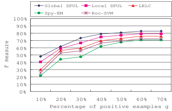
Figure 2: The performance on the Reuter-interest sub-dataset when the percentage of positive examples ( g ) increases.
