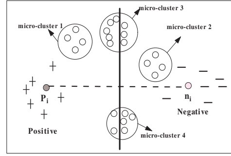
Figure 1: Illustration of similarity weight assignment to the micro-clusters in the local generation scheme. “+” represents the positive example. “-” denotes the reliable negative example. “o” stands for the ambiguous example.)
