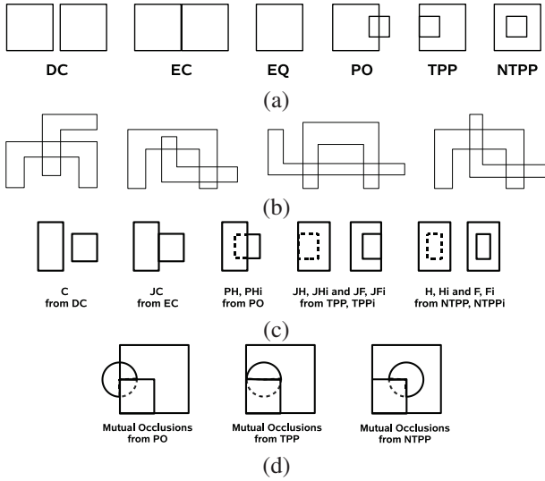
Figure 3: Illustrating the region connection relations – (a) Six of the RCC-8 region connection relations (inverses of TPP and NTPP are excluded). (b) The multiply connected spatial arrangements that are manifested by the same relation PO . (c) Schematic diagrams of the LOS-14 relations, (excluding EH and EH i ) [Galton, 1994]. (d) The Mutual occlusion relations from ROC-20 [Randell et al. , 2001] (inverse relations and equality excluded).
