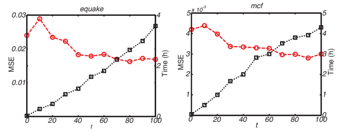
Figure 4: Prediction accuracies (MSE) and computational costs (Time) of COMT with respect to different numbers of training iterations ( t ).
