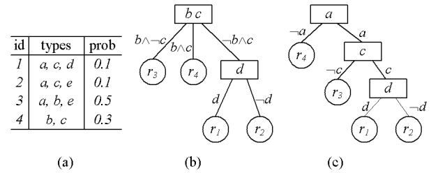
Figure 2: Two decision trees, (b) and (c), for exploring the database (a).
