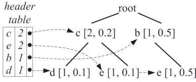
Figure 5: The FP-Tree indexing \mathbb{R}^a in Figure 2.
