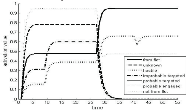
Figure 9: Complex belief activations for scenario 2
