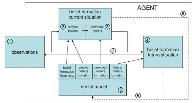
Figure 1: Cognitive model for situation awareness: overview
