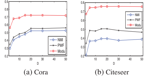
Figure 4: Sensitivity to the parameter D of GLFM.
