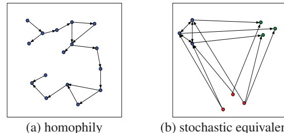
Figure 1: Homophily and stochastic equivalence in networks.
